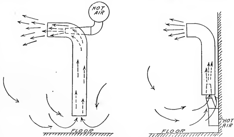
FIG. 14. TWO FORMS OF THE "CIRCULATING OUTLET". A PATENTED DEVICE FOR IMPROVING THE WARM AIR DISTRIBUTION IN CONNECTION WITH A FAN SYSTEM
